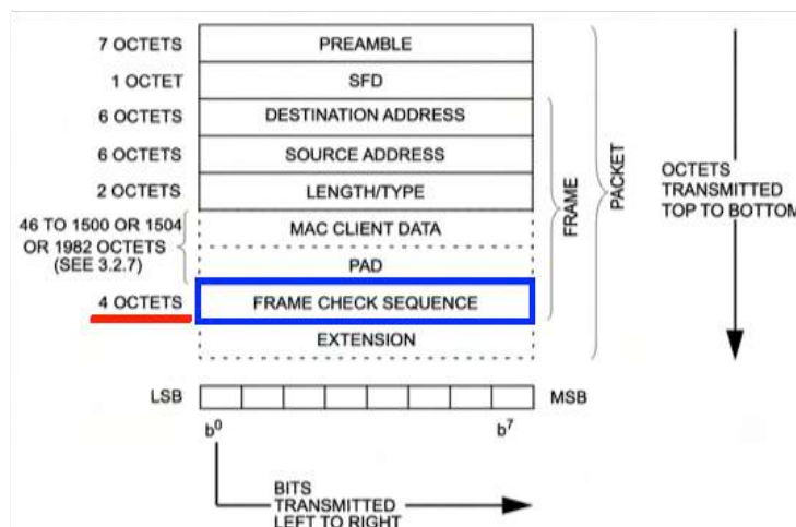
Figure 3-1—Packet format
